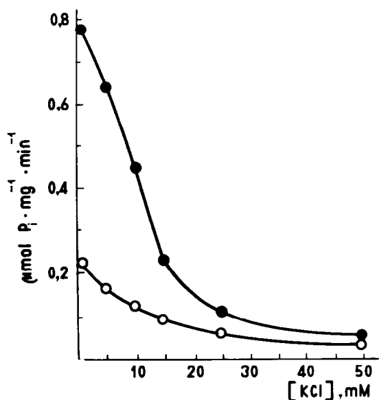
Fig.3. Effect of different concentrations of \text{KCl} on the actin-stimulated \text{Mg}^{2+} -ATPase activity of myosin minifilaments with phosphorylated \text{LC}_2 (●) and dephosphorylated \text{LC}_2 (○). Other conditions as in fig.1.
